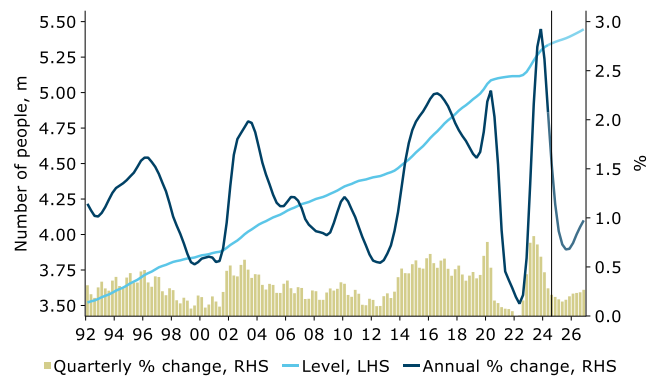
Figure 16. Employment
